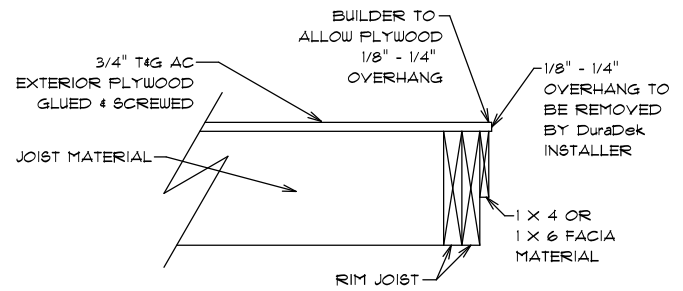
DECK CONSTRUCTION: STEP 1
